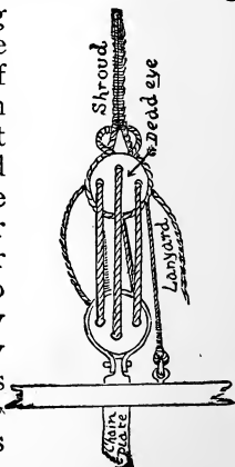
SHROUD, DEADEYE, LANYARD.
